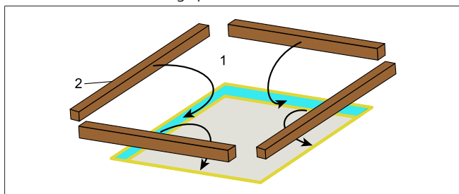
Fig. 7 Roof reinforcement
