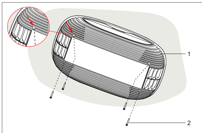
Fig. 25 Fixing the air distributor assembly to the mounting bracket
