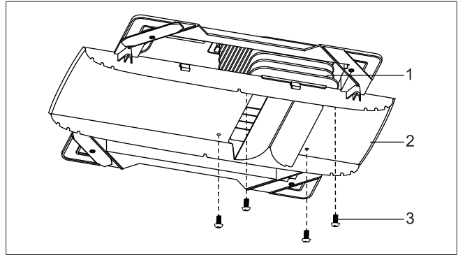
Fig. 21 Connecting the air outlet duct
