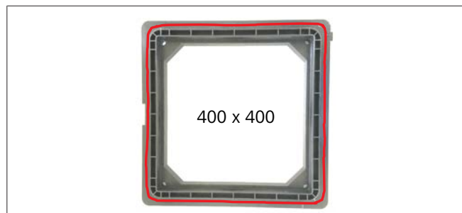
Fig. 11 Sealant path
