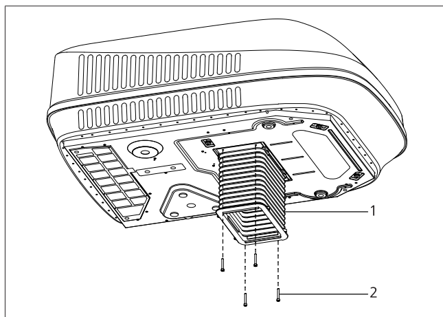
Fig. 18 Installing the air inlet duct
