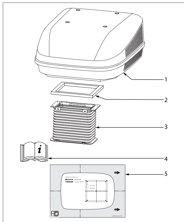
Fig. 1 Outdoor unit
