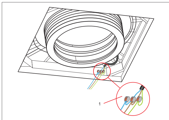
Fig. 19 Location of the terminal blocks
