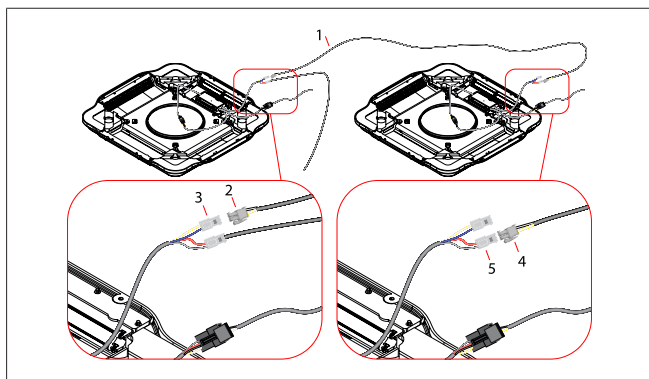
Fig. 26 Connecting two CI-BUS units
