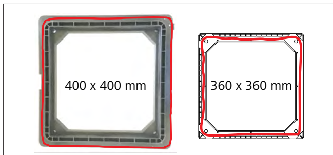
Fig. 16 Sealant paths
